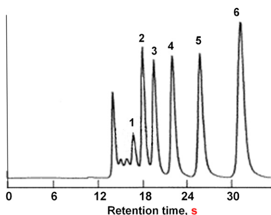
Fig. 2. Reversed phase separation of alkylbenzenes using monolithic C18 silica column. Conditions: column 8.3 \text{ cm} \times 7 \text{ mm} I.D., mobile phase 80% aqueous methanol, linear flow velocity 4.99 mm/s. Peaks (1) benzene, (2) toluene, (3) ethylbenzene, (4) propylbenzene, (5) butylbenzene, (6) pentylbenzene. Adapted from Ref. [4] with permission.
