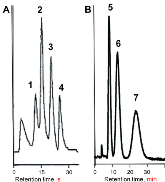
Fig. 1. Reversed-phase separations of proteins (A) and alkylbenzenes (B) using monolithic poly(styrene-co-divinylbenzene) columns. Conditions: (A) column 50 \times 8 mm I.D., mobile phase linear gradient from 20 to 60% acetonitrile in 0.1% aqueous trifluoroacetic acid in 24 s, flow rate 25 mL/min; (B) column 100 \times 8 mm I.D., mobile phase 70% aqueous acetonitrile, flow rate 1 mL/min. Peaks: ribonuclease A (1), cytochrome c (2), myoglobin (3), ovalbumin (4), benzene (5) ethylbenzene (6), butylbenzene (7).
