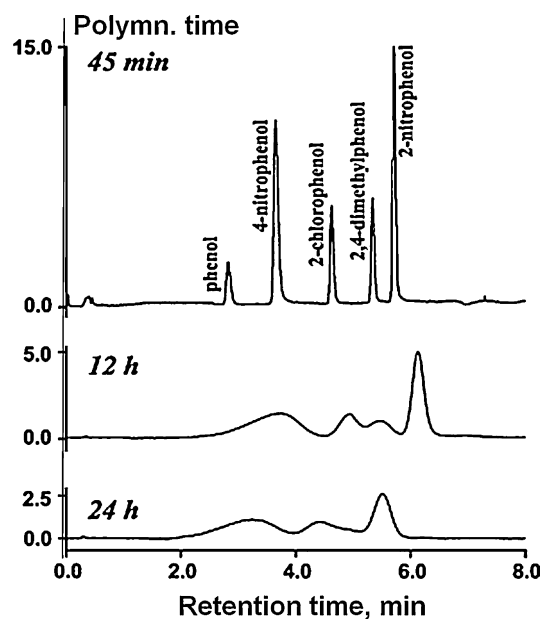
Fig. 10. Separation of phenol derivatives using monolithic poly(4-methylstyrene- co -1,2-bis-(4-vinylphenyl)ethane) capillary column polymerized for varying times. Conditions: column 80 mm \times 0.2 mm I.D., mobile phase A: 0.1% aqueous trifluoroacetic acid, B: 0.1% trifluoroacetic acid in acetonitrile, gradient 0–50% B in A in 5 min, flow rate 10 \mu L/min, UV detection at 210 nm. Adapted from Ref. [40] with permission.
