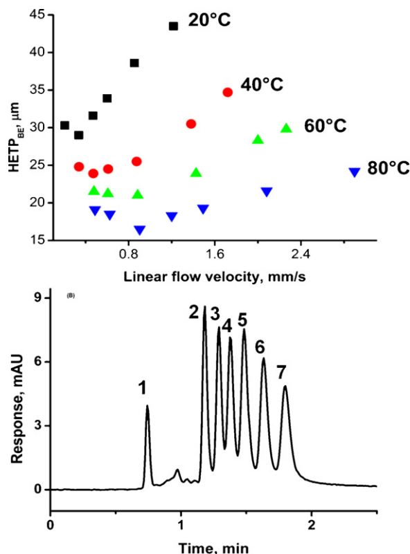
Fig. 17. Effect of temperature on van Deemter plots for benzene (A) and separation of small molecules (B) using hypercrosslinked monolithic column. Conditions: column 130 mm × 100 µm I.D., ternary mobile phase 20% water, 20% tetrahydrofuran, 60% acetonitrile, (B) flow rate 0.5 µL/min; temperature 80 °C; UV detection 254 nm; back pressure 26 MPa. Analytes: (1) uracil, (2) benzene, (3) toluene, (4) ethylbenzene, (5) propylbenzene, (6) butylbenzene, (7) pentylbenzene. Adapted from Ref. [63].
