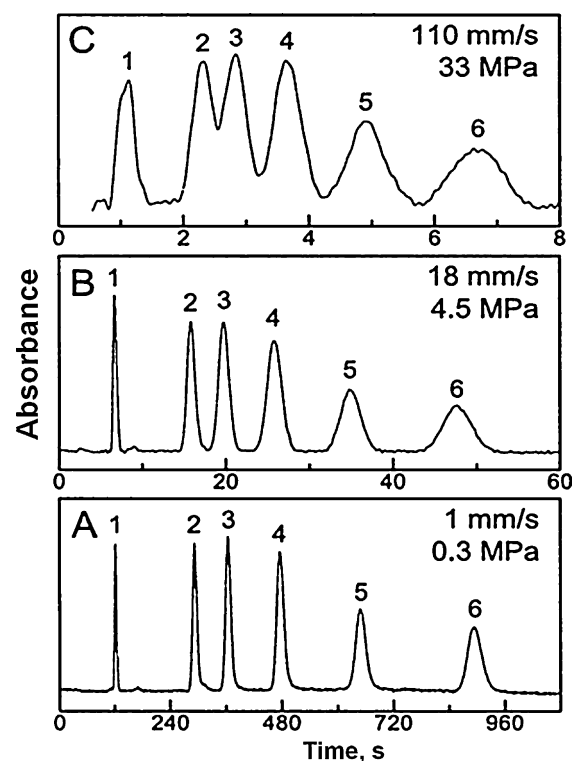
Fig. 5. Reversed phase separation of alkylbenzenes using monolithic poly(butyl methacrylate-co-ethylene dimethacrylate) capillary column prepared by UV initiated polymerization at 0 °C. Conditions: column 100 mm \times 100 \mu m I.D.; mobile phase 50% aqueous acetonitrile, UV detection at 217 nm. For flow rate and back pressure see inserts. Peaks: uracil (1), toluene (2), ethylbenzene (3), propylbenzene (4), butylbenzene (5), pentylbenzene (6). Reproduced from Ref. [15] with permission.
