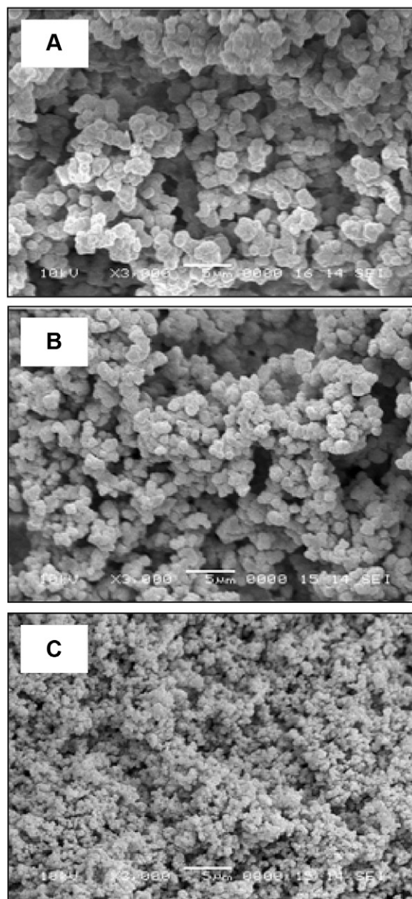
Fig. 8. Scanning electron micrographs of monolithic poly(butyl methacrylate-co-ethylene dimethacrylate) polymers prepared in a 320 \mu\text{m} I.D. capillary using mixtures consisting of 1-propanol 1,4-butanediol, and water as a porogen. Compositions of porogen:water 10% 1-propanol-1,4-butanediol 60:30 (A), 62:28 (B), 64:26 (C).
