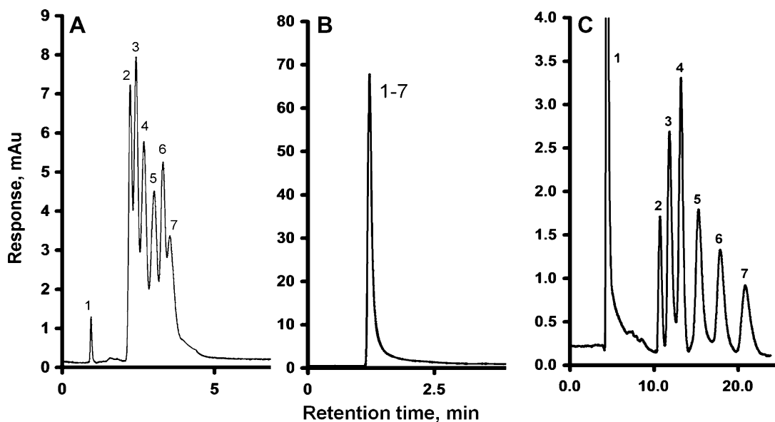
Fig. 19. Separation of uracil and alkylbenzenes using a monolithic poly(glycidyl methacrylate-co-ethylene dimethacrylate) capillary column (A), the previous column reacted with ammonia (B), and column modified with oxidized carbon nanotubes (C). Conditions: (A) column, 180 mm \times 100 \mu\text{m} I.D., mobile phase 45% acetonitrile–5% THF–50% water, flow rate 1.00 \mu\text{L}/\text{min} , back pressure 16 MPa; (B) column, 200 mm \times 100 \mu\text{m} I.D., mobile phase 50% acetonitrile–50% water, flow rate 1.00 \mu\text{L}/\text{min} , back pressure 17 MPa; (C) column, 170 mm \times 100 \mu\text{m} I.D., mobile phase 47.5% acetonitrile–2.5% THF–50% water mixture; flow rate 0.25 \mu\text{L}/\text{min} , back pressure 30 MPa. Peaks: uracil (1), benzene (2), toluene (3), ethylbenzene (4), propylbenzene (5), butylbenzene (6), and amylbenzene (7). Adapted from Ref. [93].
