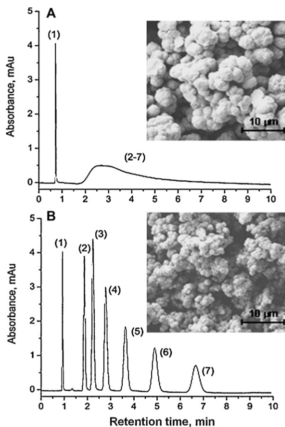
Fig. 12. Isocratic separation of alkylbenzenes using monolithic poly(butyl methacrylate-co-ethylene dimethacrylate) capillary columns polymerized for 48 (A) and 0.5 h (B) in a 100 \mu m I.D. capillary. Conditions: column 200 mm \times 100 \mu m I.D.; mobile phase: 50% aqueous acetonitrile; flow rate: 1.6 \mu L/min; linear flow velocity 4.6 mm/s (A) and 3.6 mm/s (B); back pressure 3.92 (A) and 1.14 MPa (B). Peaks: (1) uracil, (2) benzene, (3) toluene, (4) ethylbenzene, (5) propylbenzene, (6) butylbenzene, (7) pentylbenzene. Inlay SEM micrographs show morphology of the monoliths. Adapted from Ref. [42] with permission.
