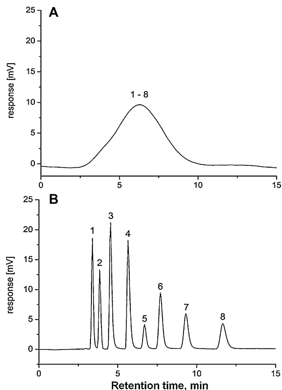
Fig. 7. Separation of small organic molecules using poly(styrene-co-divinylbenzene) (A) and poly(styrene-co-methacrylic acid-co-divinylbenzene) (B) columns. Conditions: mobile phase, acetonitrile/water (65/35, v/v); UV detection at 214 nm; flow rate, 4 \mu\text{L}/\text{min} ; injection volume, 100 nL; column 170 mm \times 320 \mu\text{m} I.D. Peaks: thiourea (1), phenol (2), aniline (3), benzene (4), toluene (5), ethylbenzene (6), propylbenzene (7), butylbenzene (8). Reproduced from Ref. [24] with permission.
