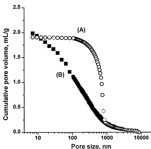
Fig. 4. Integral pore size distribution profiles of poly(styrene-co-divinylbenzene) monoliths prepared by a polymerization at different temperatures. Conditions: (A) polymerization mixture styrene 20 wt.%, divinylbenzene 20 wt.%, 1-dodecanol 40 wt.%, toluene 20 wt.%, benzoyl peroxide 0.5 wt.% (with respect to monomers), temperature 70 °C, reaction time 24 h; (B) polymerization mixture styrene 20 wt.%, divinylbenzene 20 wt.%, 1-dodecanol 60 wt.%, benzoyl peroxide 0.5 wt.% (with respect to monomers), temperature 130 °C, reaction time 8 h.
